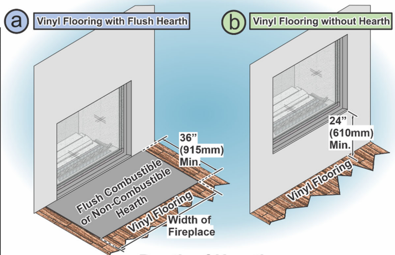
Depth of Hearth
